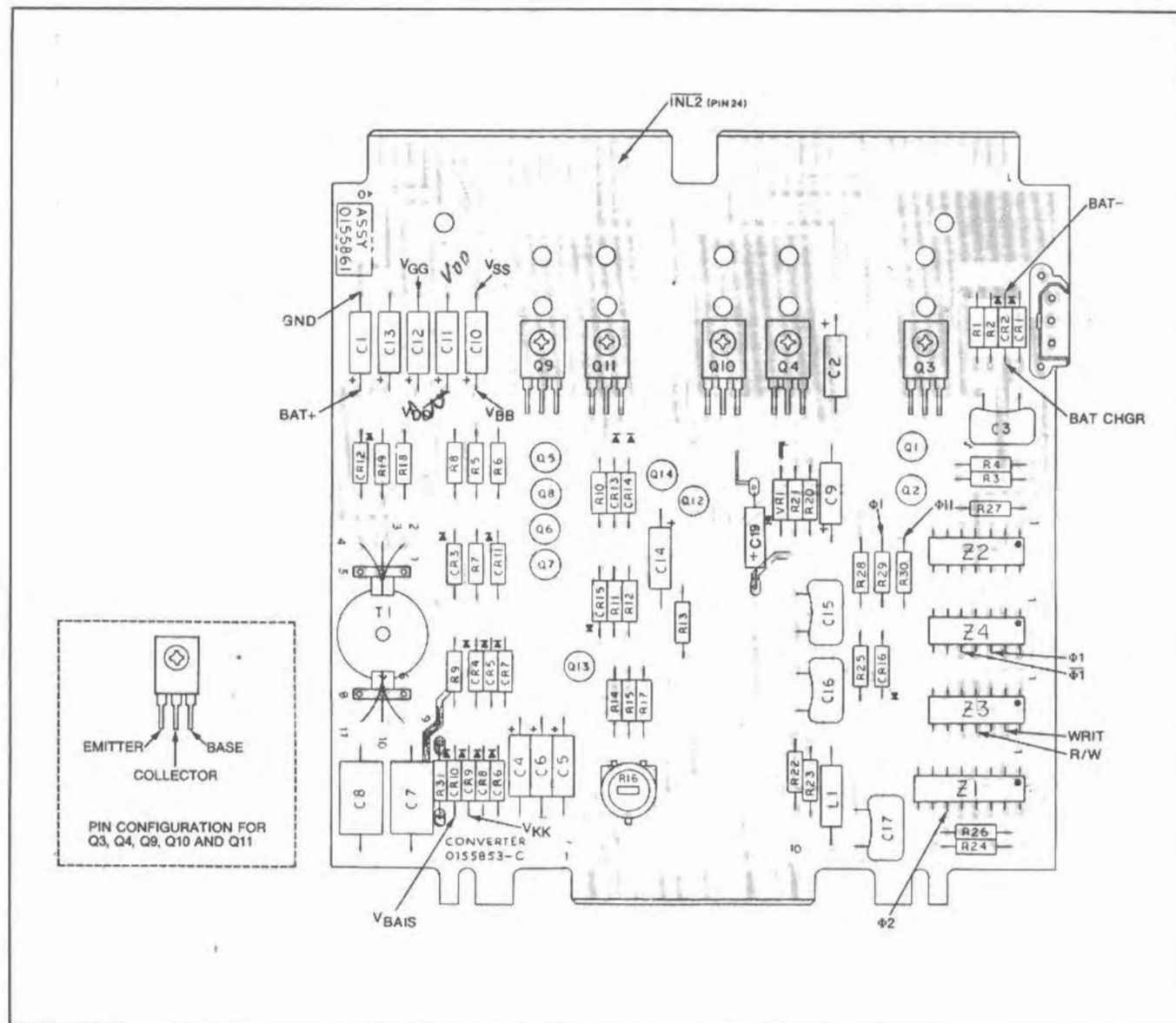
Fig. 7-2 Converter Board, Typical Test Points
