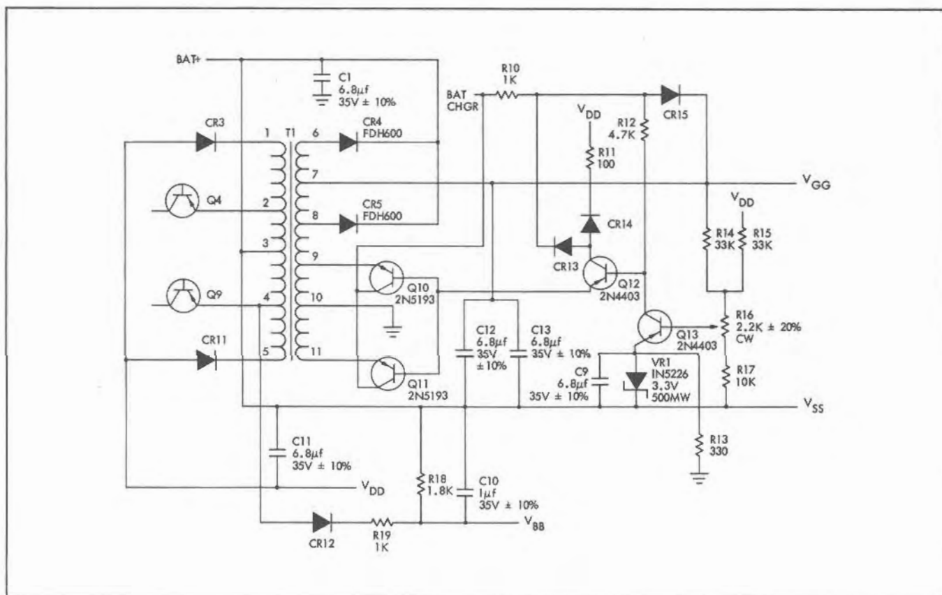
Fig. 2-6 Low Voltage Supply Schematic
