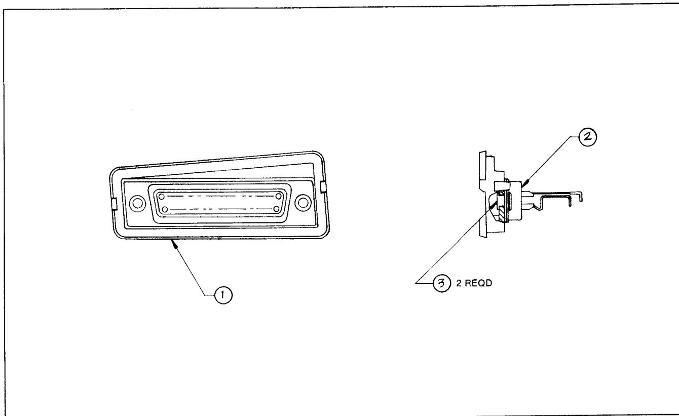
Fig. 12-13 I/O Connector Assembly (Assembly Number 0157073)
