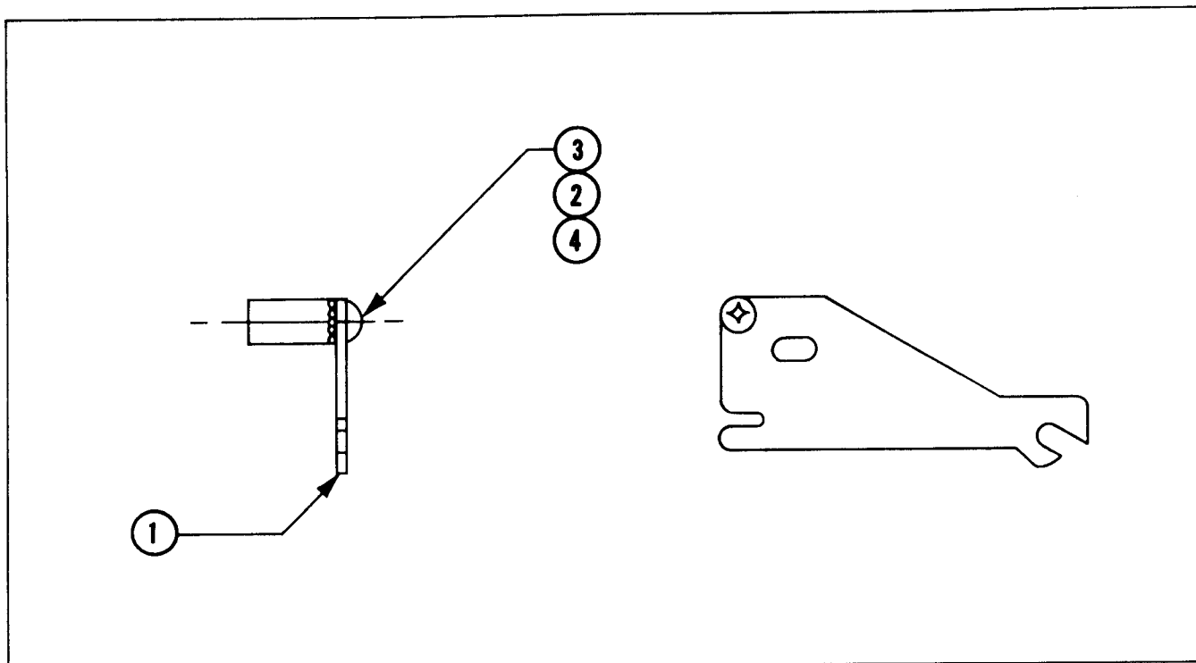
Fig. 12-6 Right Latch Plate Assembly (Assembly Number 0141077)
