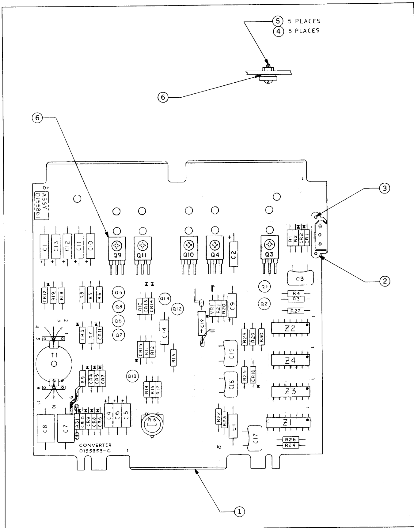
Fig. 12-11 Converter Board Assembly (Assembly Number 0155861)
