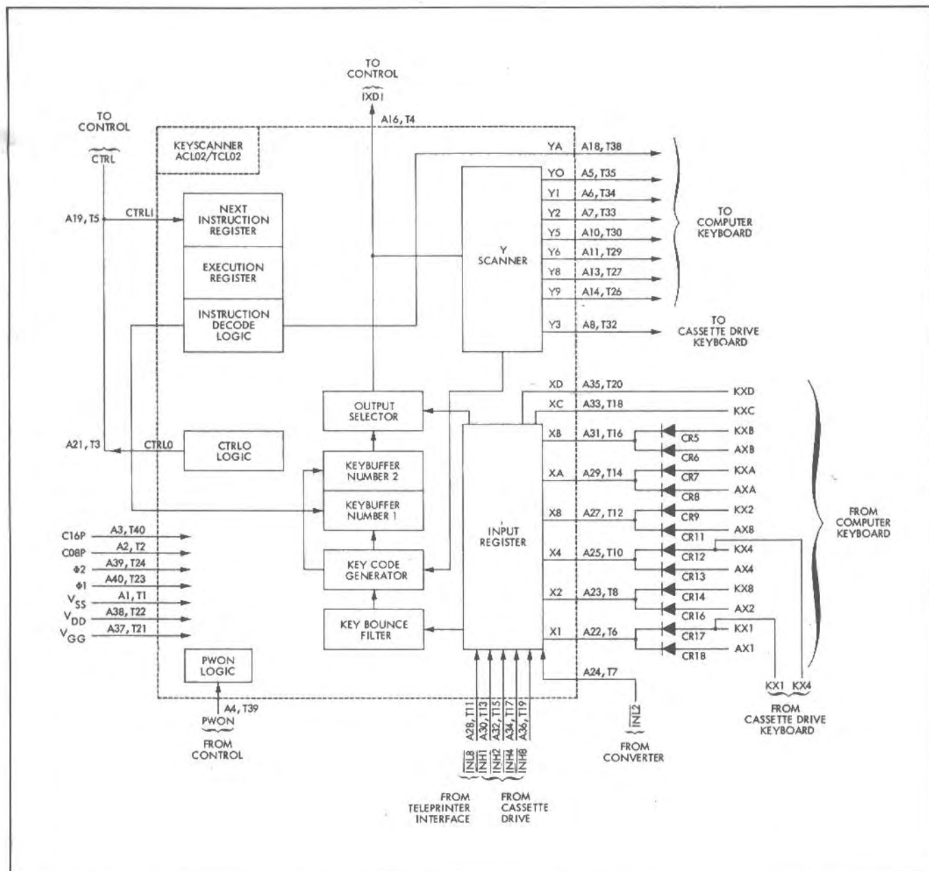
Fig. 2-11 Keyscanner Schematic
