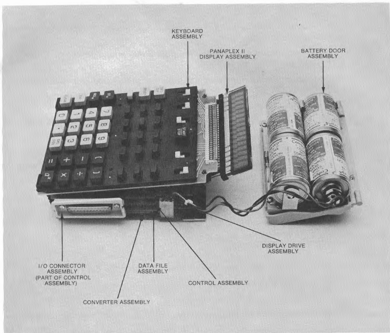
Fig. 1-2 Major Assemblies
