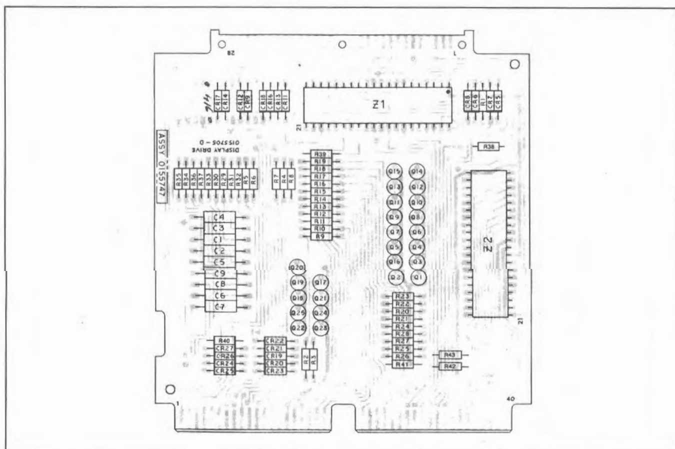
Fig. 9-1 Display Drive Board
