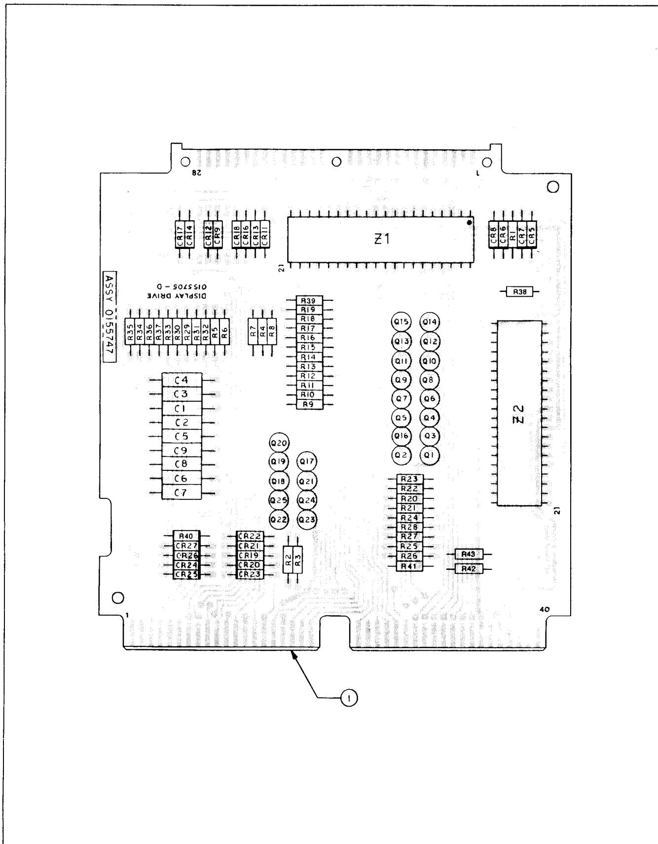
Fig. 12-14 Display Drive Assembly, ACL Version (Assembly Number 0155747)
