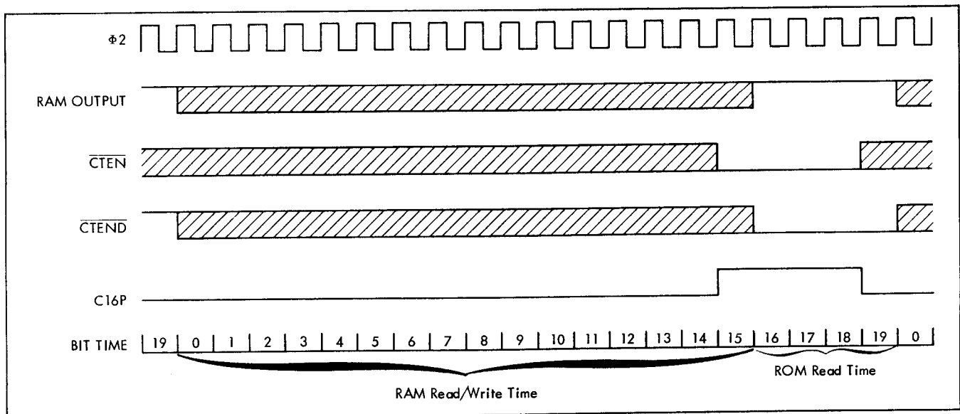
Fig. 11-3 Data File Timing Diagram
