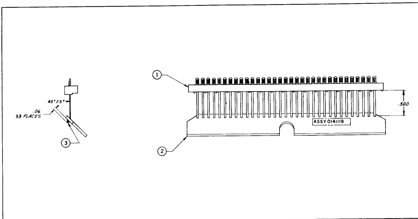
Fig. 12-9 Display Interconnect Assembly (Assembly Number 0141119)
