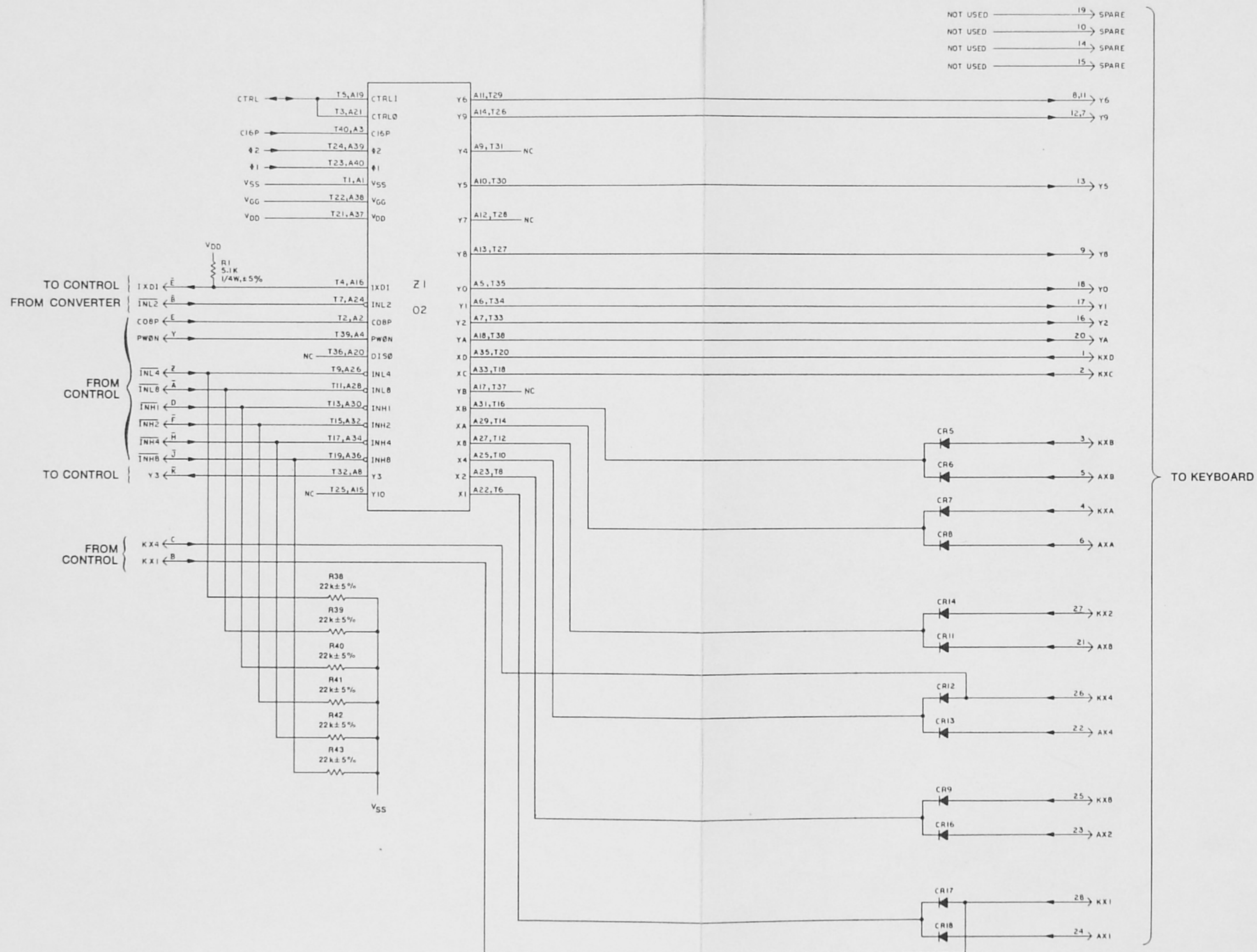
Fig. 9-3 KeyScanner Circuits, Typical Schematic Diagram
