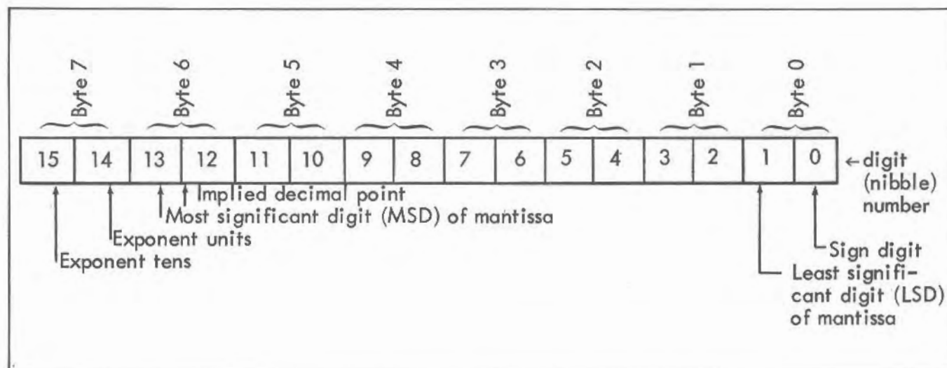
Fig. 2-15 Register Structure
