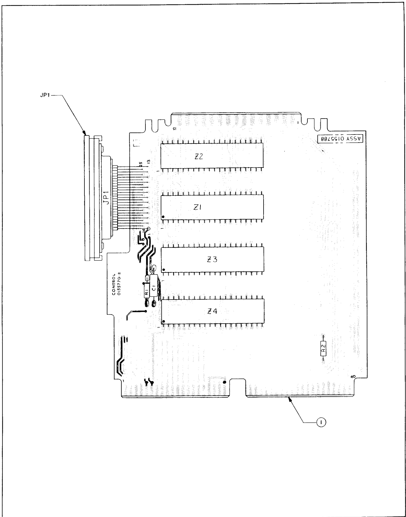
Fig. 12-12 Control Assembly, ACL Version (Assembly Number 0155788)
