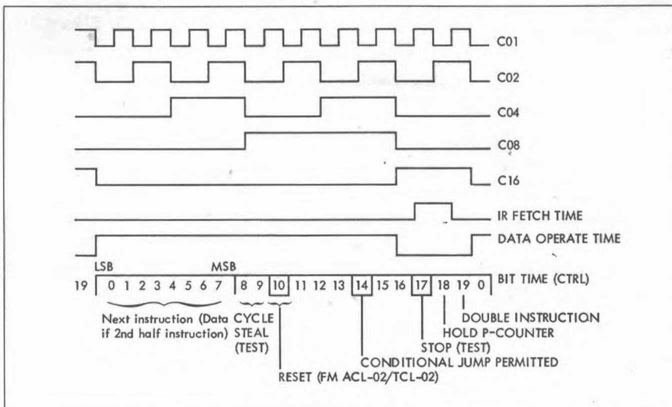
Fig. 2-23 System Timing
