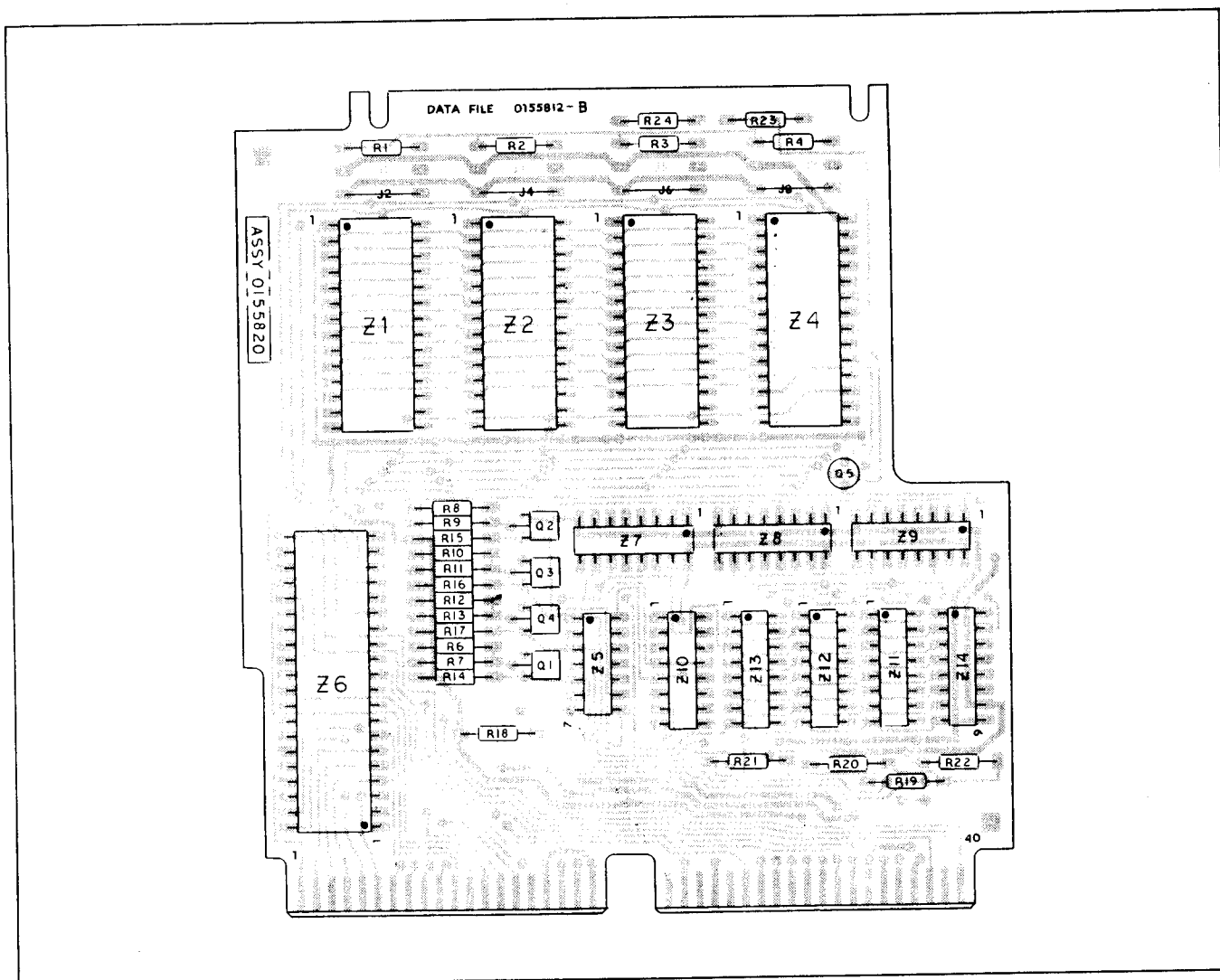
Fig. 11-1 Data File Assembly
